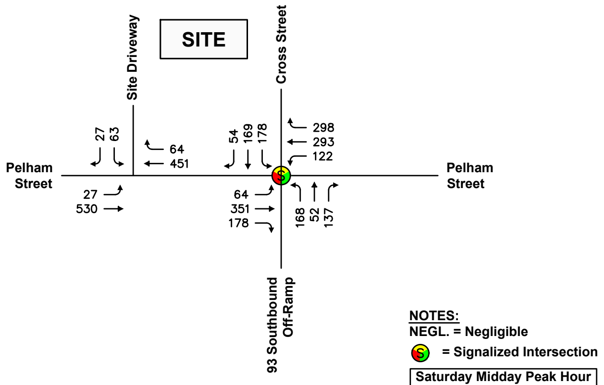
Figure 9 2023 Design Year Conditions Weekday Midday and Saturday Midday Peak Hour Traffic Volumes
